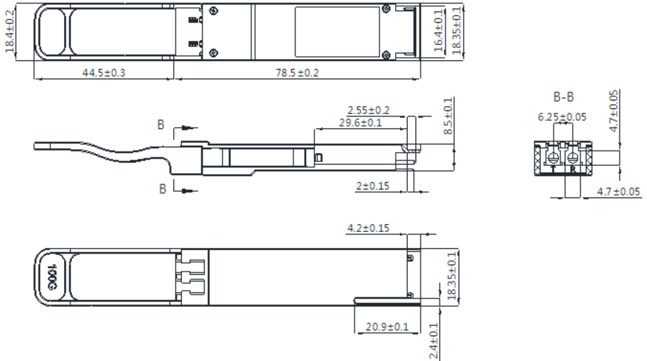
Figure 5. Outline Drawing
